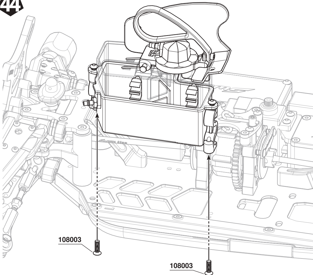
108003 M3x10mm FH/ST HEX Screw x2
