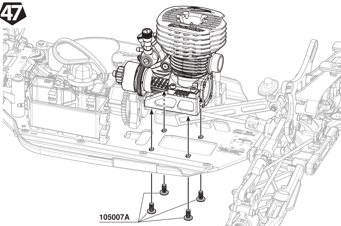
105007A M4x8mm I-Head Screw x4
