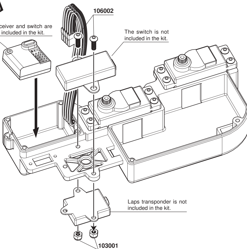
106002 M3x10mm Hex Socket OH/TP Screw x2
