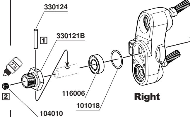
116006 Ball Bearing 8x16x5mm x4
