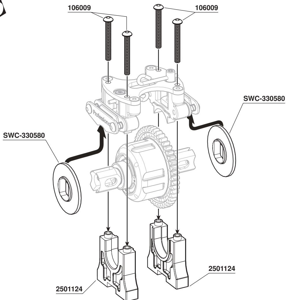
106009 M3x25mm Hex Socket OH/TP Screw x4
