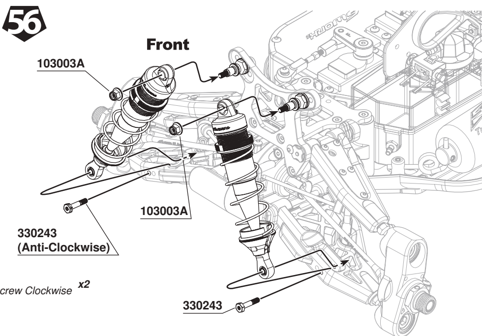
330243 SWORKz 3x16mm Shock Hex Screw Anti-Clockwise x2
